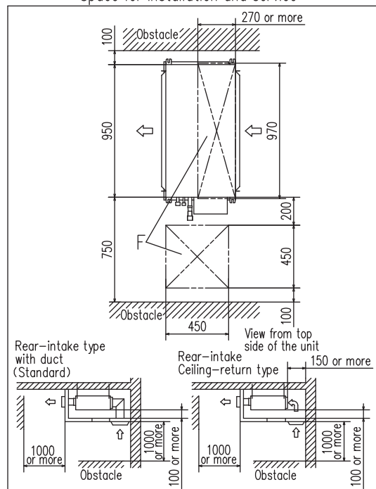
Space for installation and service
