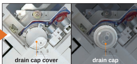
drain pump port
